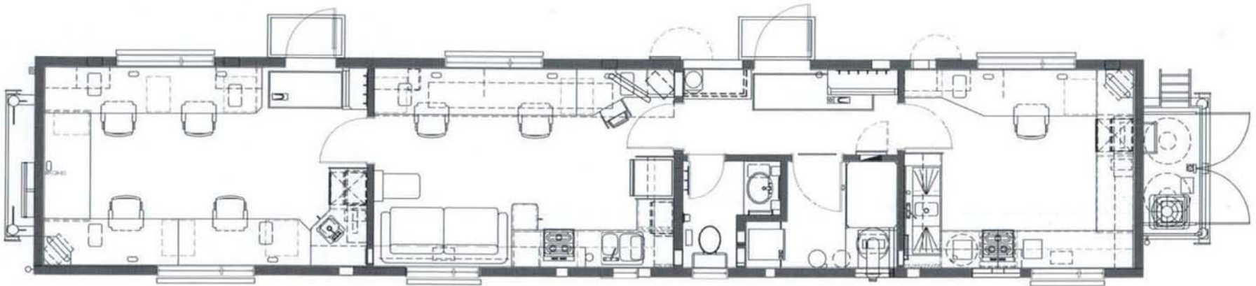
12' x 60' (skid) "DRILLING CONTROL CENTER"
